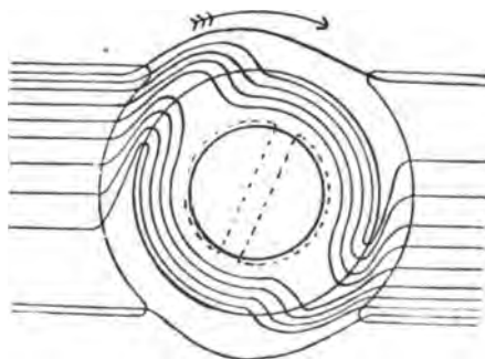
FIG. 430.—Diagram of the Distortion of the Lines of Magnetic Force as they pass through the Body of a Rotating Dynamo Armature.
